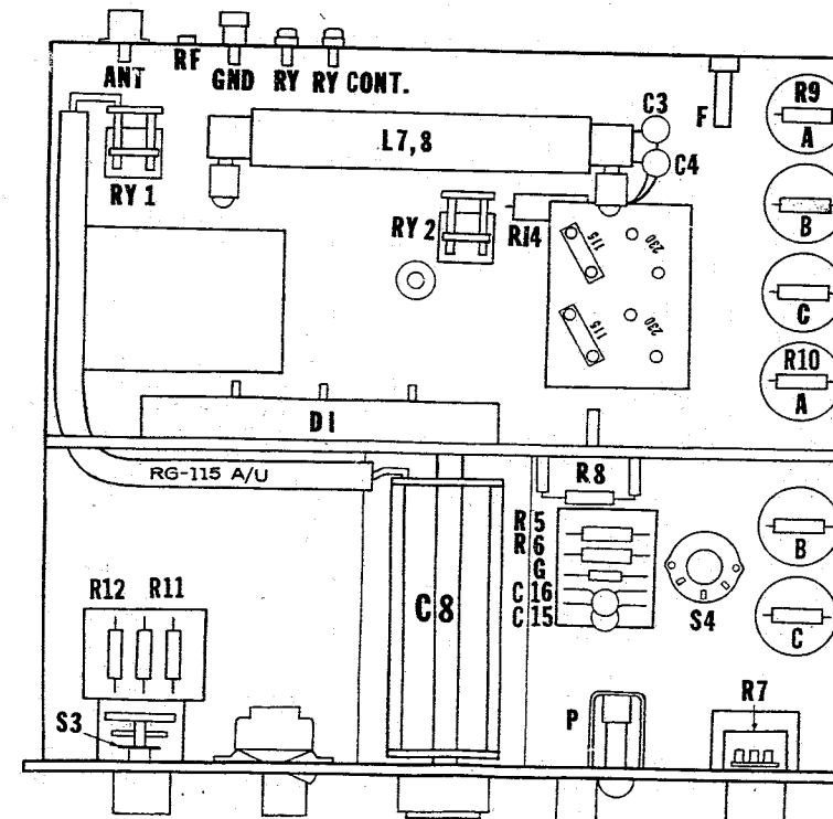
FIGURE 5 Chassis Underside
